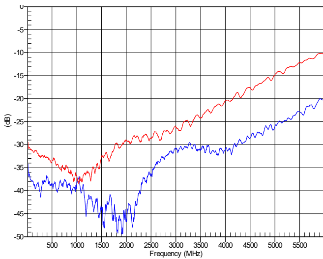
Figure 7 TX, RX Return Loss
